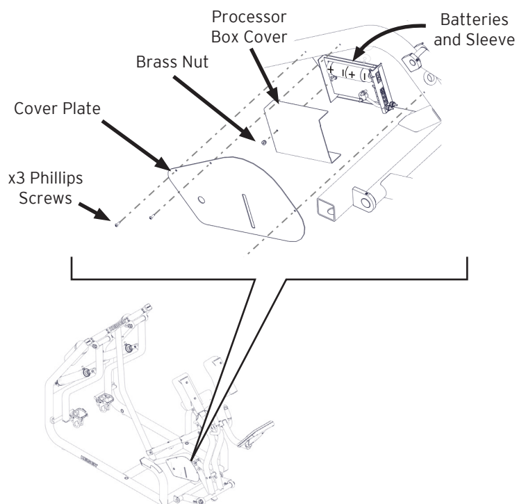
Figure 12. Battery Replacement
